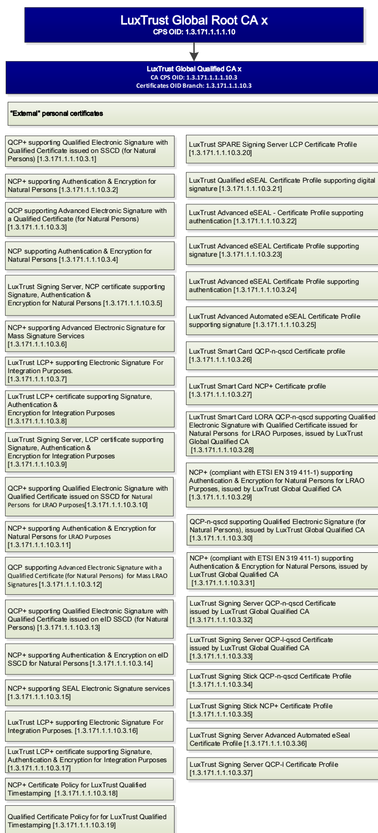
Figure 3 - LuxTrust Global Qualified CA Hierarchy
